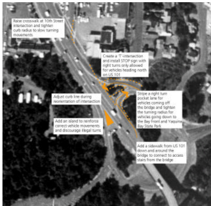
Figure 3-2. Recommended Improvements, North Bridgehead, Yaquina Bay Bridge
