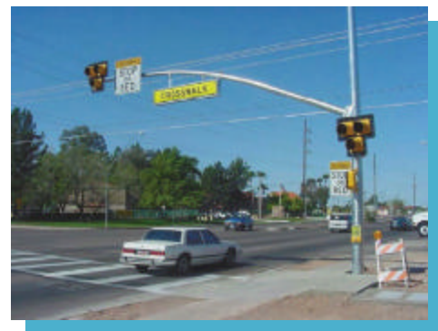
Hawk signal
