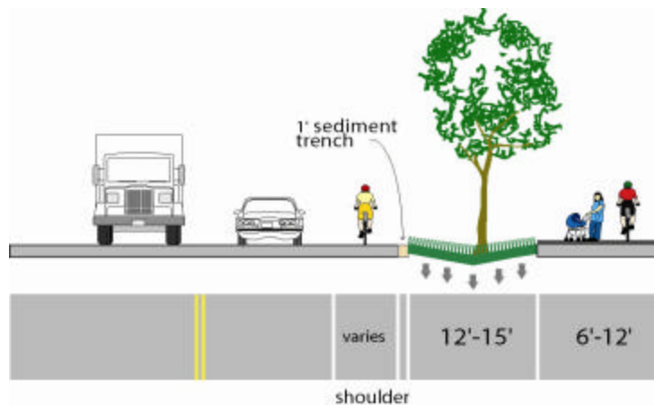
Figure 5-9. Bio-swale
