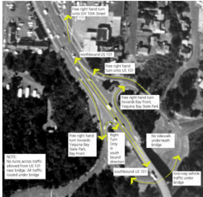
Figure 3-1. Existing Conditions, North Bridgehead, Yaquina Bay Bridge
