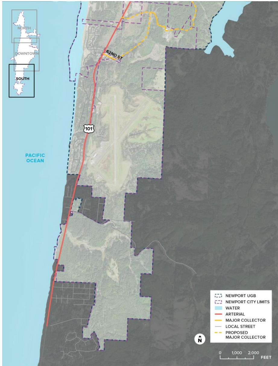
FIGURE 24: FUNCTIONAL CLASSIFICATIONS (SOUTH)
