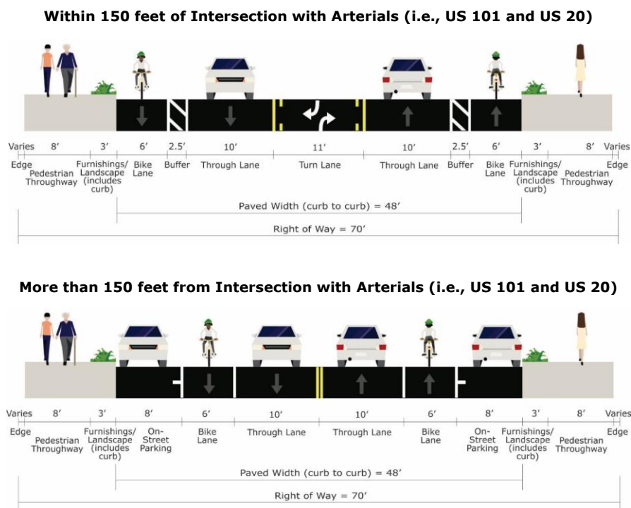
FIGURE 30: CITY MAJOR COLLECTOR (COMMERCIAL AREA) CROSS-SECTION
