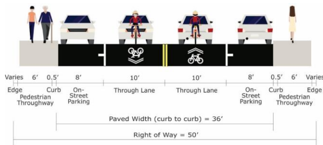
FIGURE 32: CITY NEIGHBORHOOD COLLECTOR CROSS-SECTION
