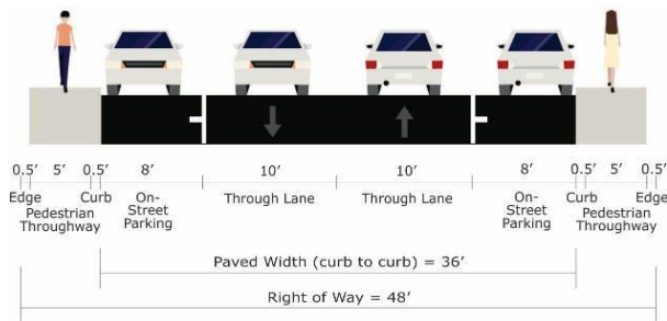
FIGURE 33: CITY LOCAL STREET CROSS-SECTION
