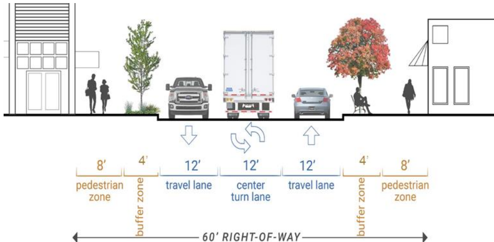
FIGURE 39: PREFERRED US 20 CIRCULATION OPTION
