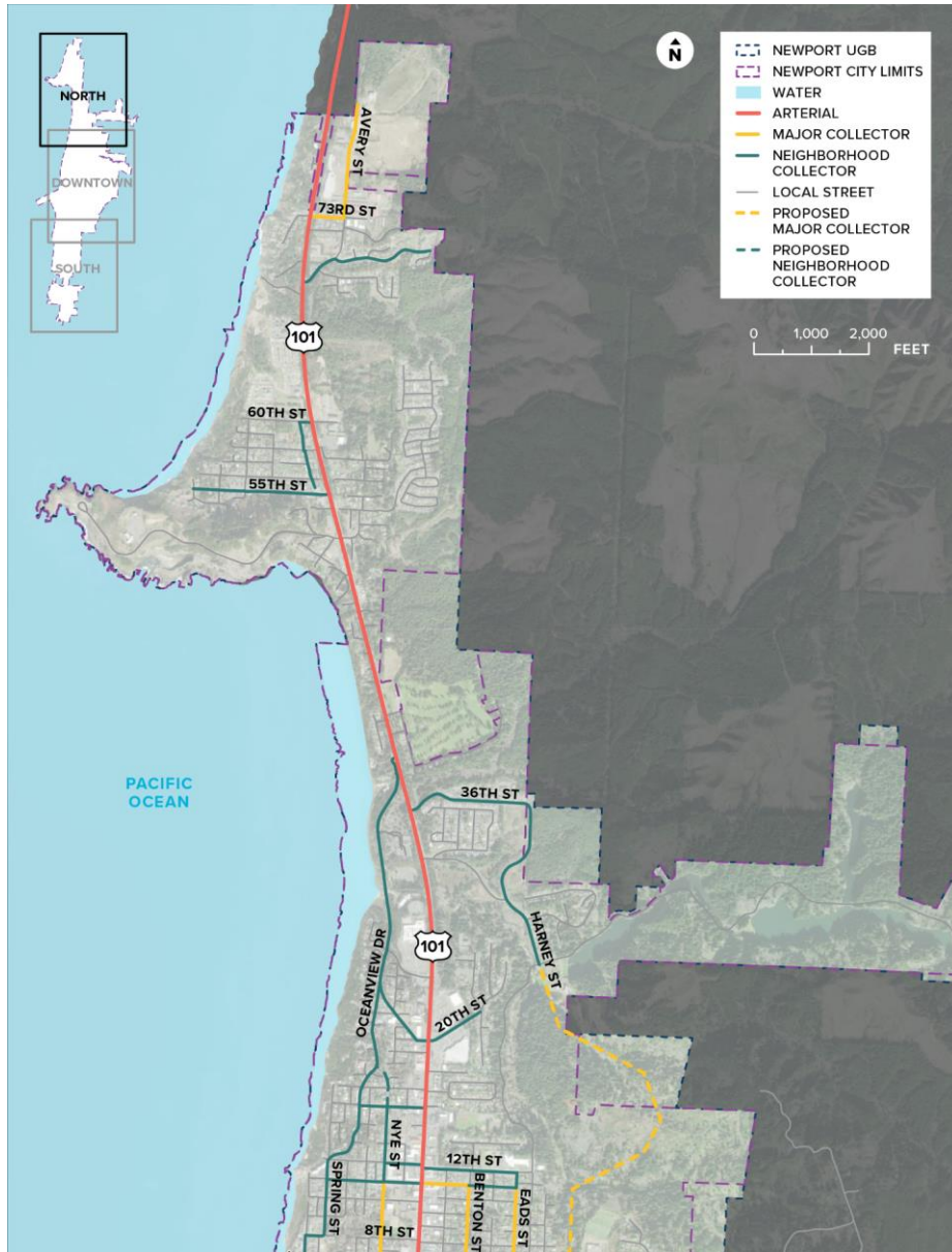
FIGURE 22: FUNCTIONAL CLASSIFICATIONS (NORTH)
