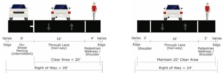
FIGURE 35: CITY LOCAL SHARED STREET CROSS-SECTION
