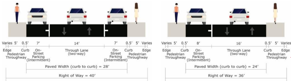
FIGURE 34: CITY LOCAL YIELD STREET CROSS-SECTION
