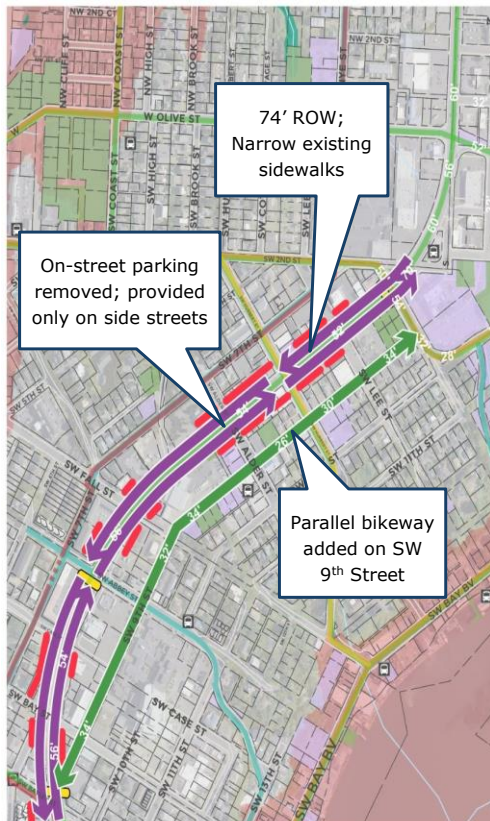
FIGURE 38: US 101 TWO-WAY CIRCULATION OPTION
