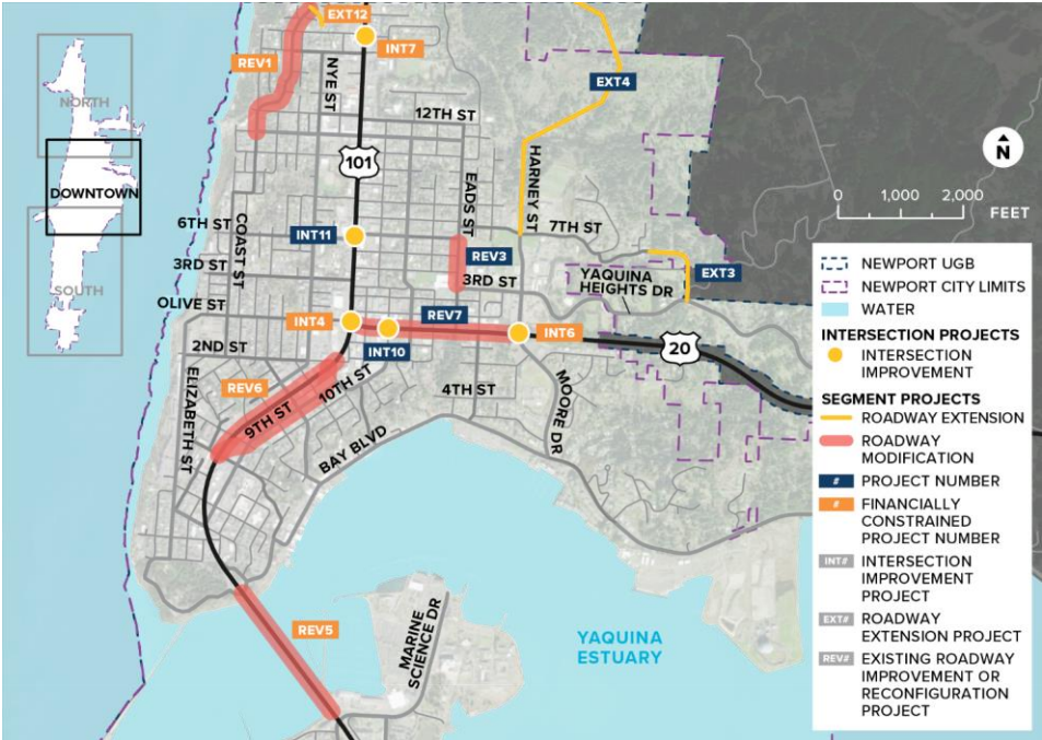
FIGURE 45: ASPIRATIONAL MOTOR VEHICLE PROJECTS (DOWNTOWN)
